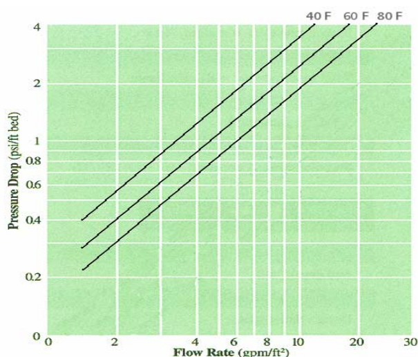
Pressure Loss Curve
